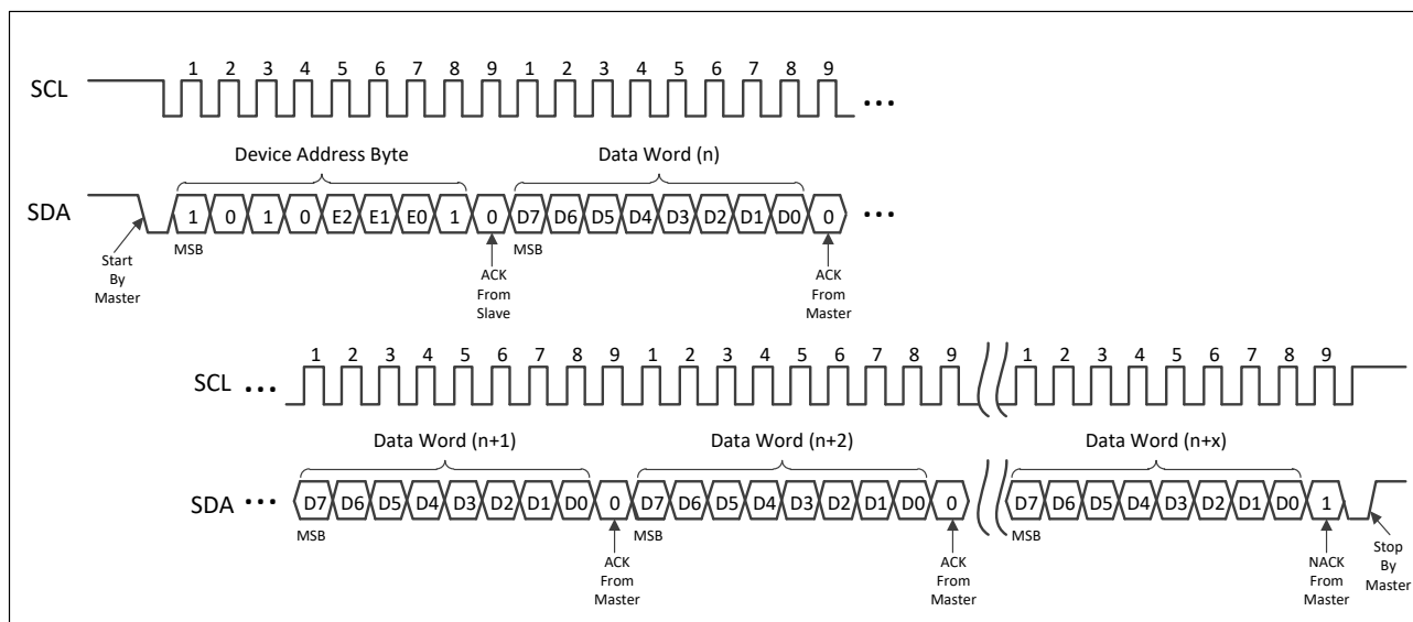
Figure 5–11 Sequential Read
