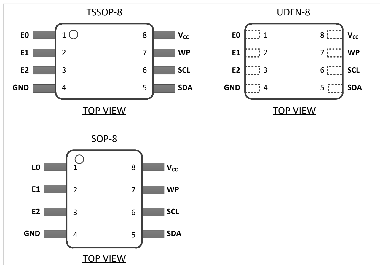
Figure 1–1 Pin Configuration
