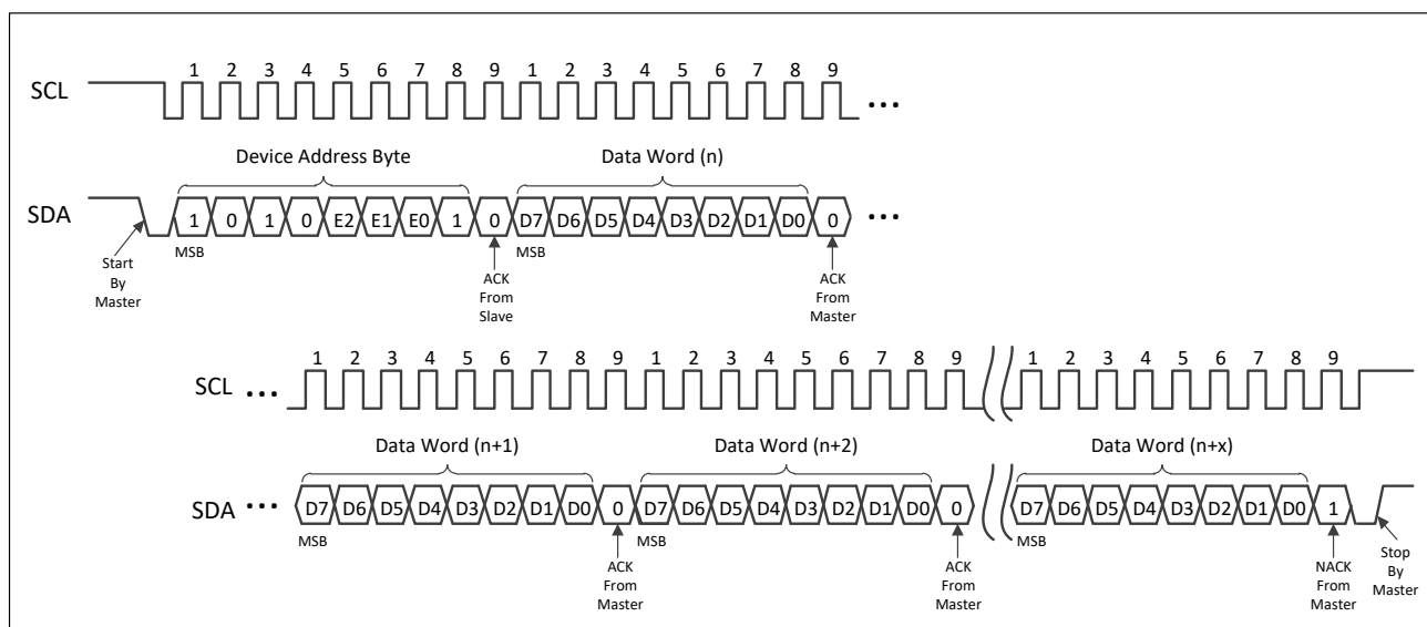
Figure 5–11 Sequential Read
