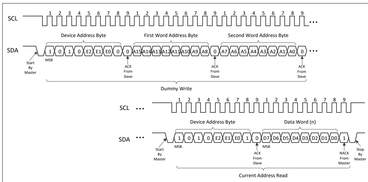
Figure 5–10 Random Read
