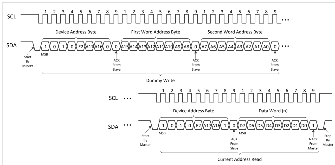
Figure 5–11 Random Read
