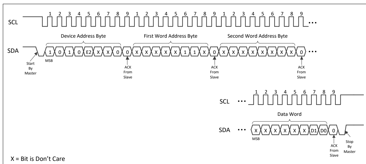
Figure 5–9 Write Software Write Protection Register
