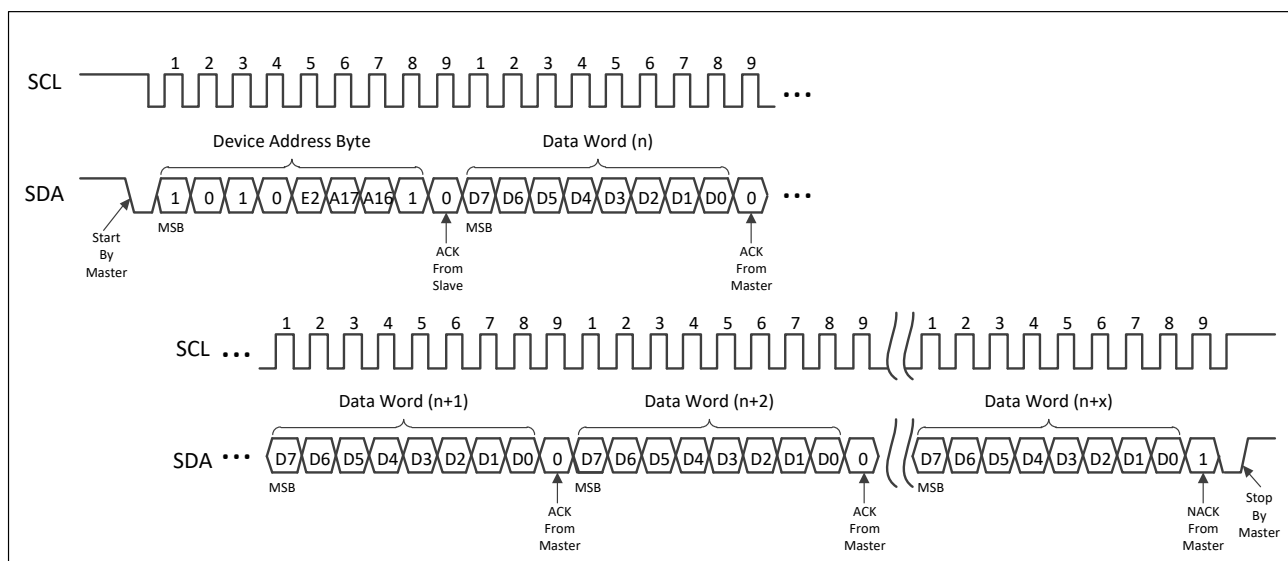
Figure 5–12 Sequential Read
