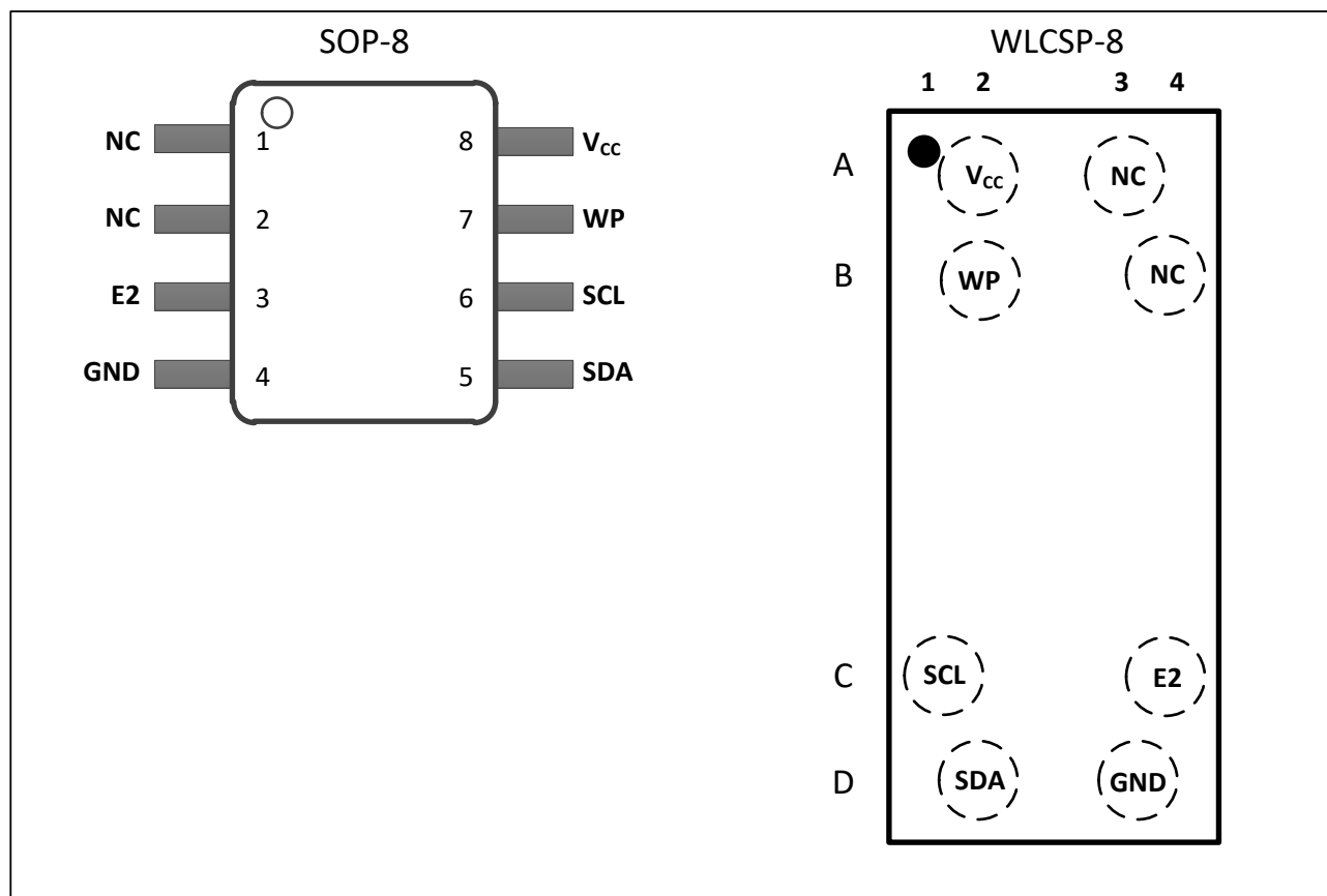
Figure 1–1 Pin Configuration (Top View)
