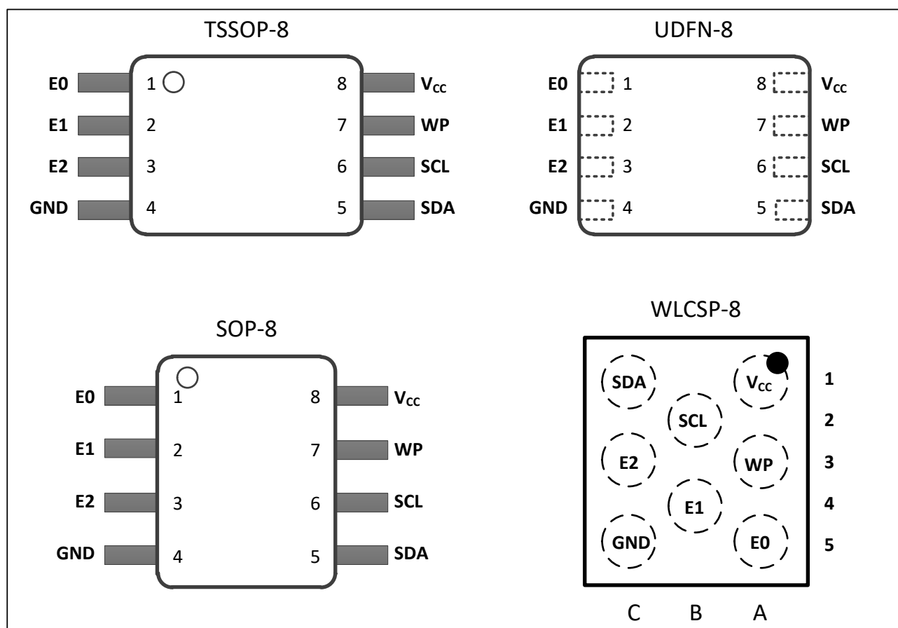
Figure 1–1 Pin Configuration (Top View)
