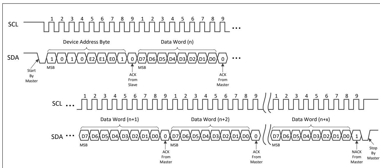
Figure 5–11 Sequential Read
