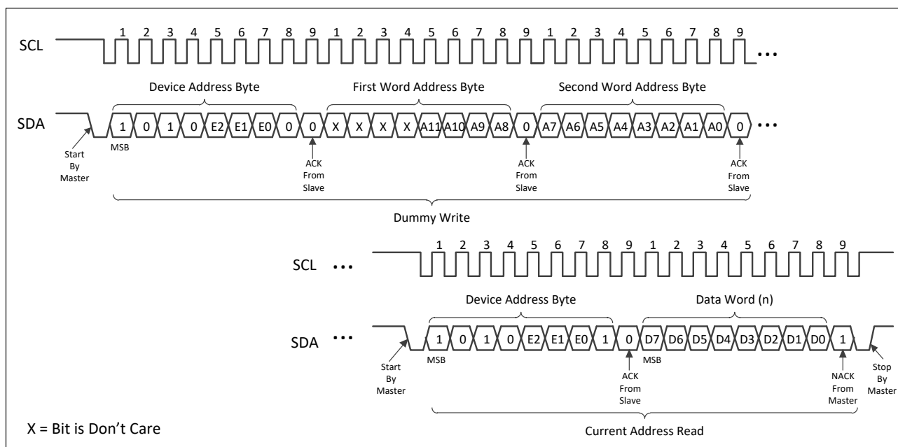
Figure 5–10 Random Read
