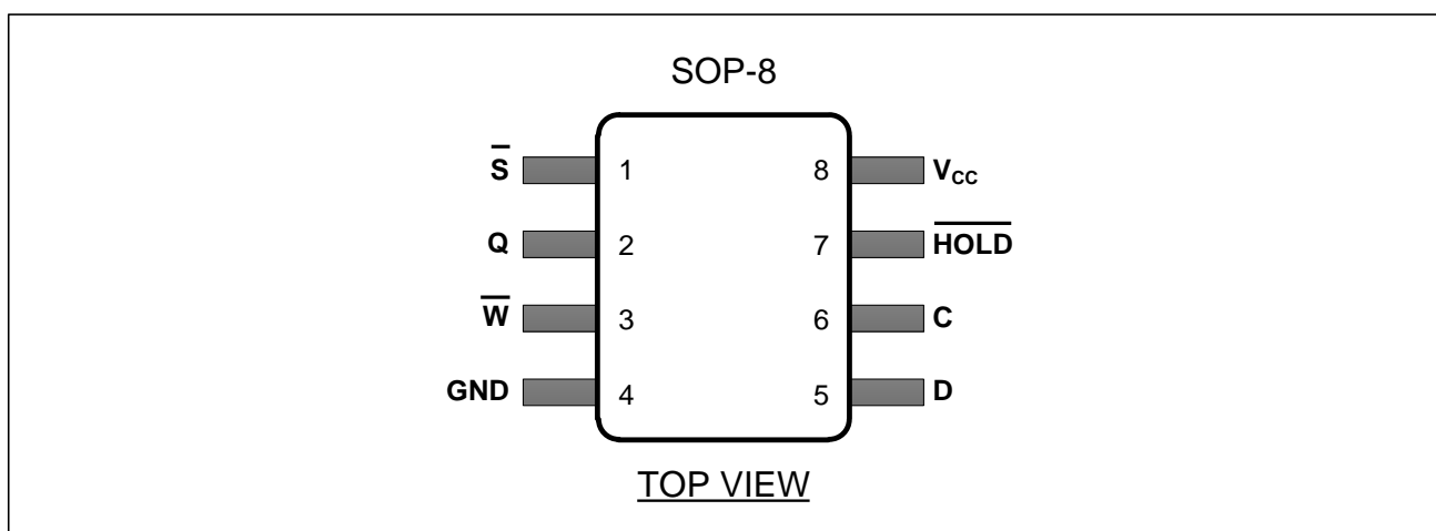
Figure 1–1 Pin Configuration
