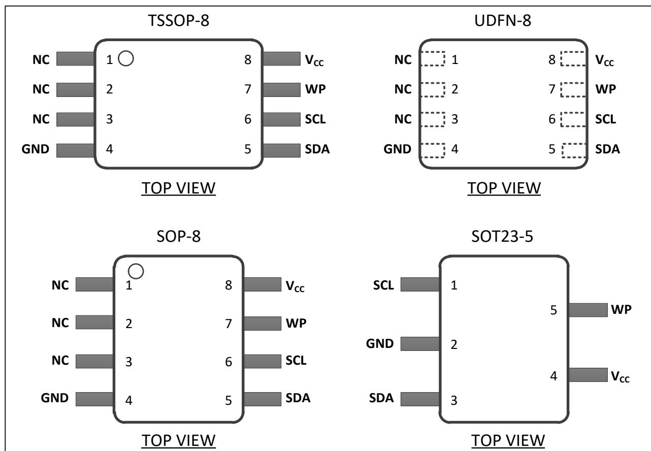
Figure 1–1 Pin Configuration
